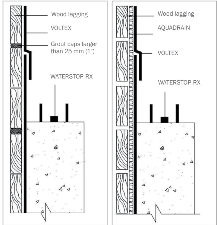
Figure 2.7 - VOLTEX installed directly to wood lagging with gaps filled. (Cast-in-place concrete wall)
