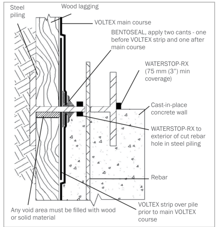
Figure 2.12 - Lagging secured to inside surface of back pile flange. Install BENTOSEAL and VOLTEX strip prior to main VOLTEX course and inward BENTOSEAL cant. (Plan View).
